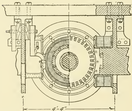
Fig. 248. End Section of New York Central Motor
